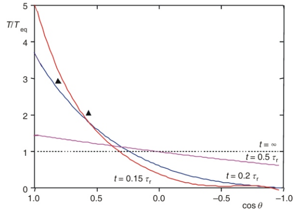
Figure 1. Angular dependence of the temperature field of the participant zone, T , in the units of temperature of equilibrium, T_{eq} , for ratio \chi = \tau / \tau_r at various times during relaxation (for times t = 0.15 \tau_r , t = 0.2 \tau_r and t = 0.5 \tau_r ); at equilibrium ( t = \infty ) the distribution is isotropic.
